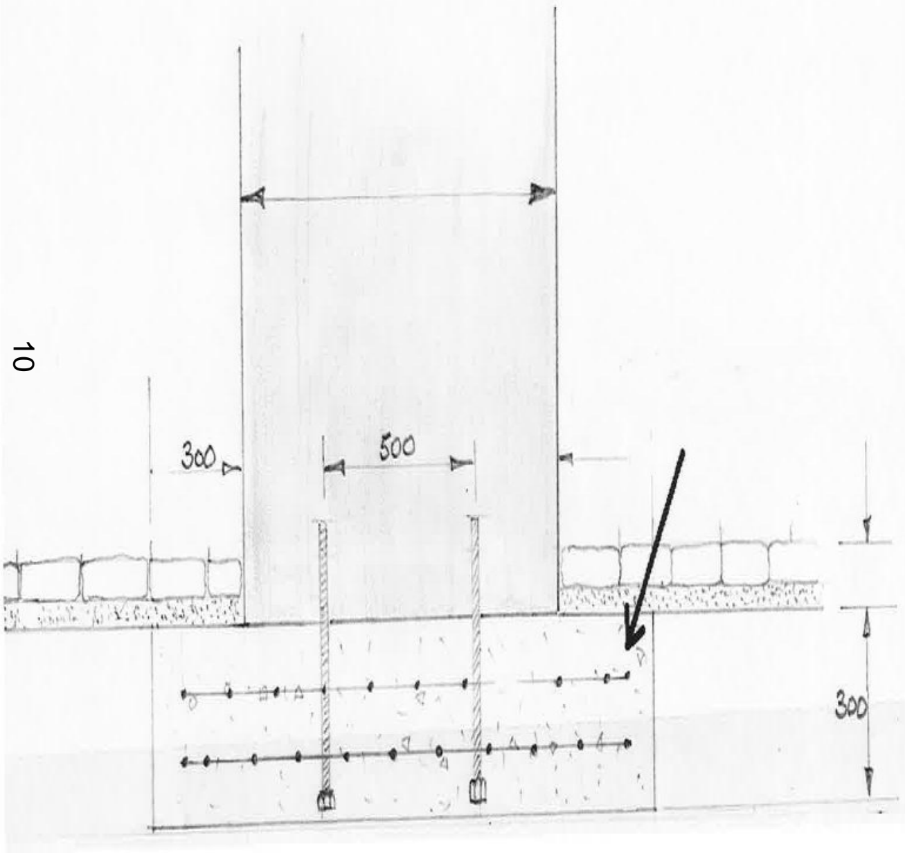
Foundation detail
